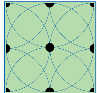
Step 3 Larger areas may require sprinklers in the middle, in addition to the sides, in order to provide head-to-head or overlapping coverage.
